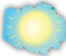
the sun
